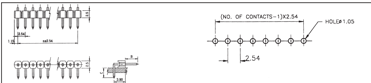
DRAWING - SINGLE ROW, RIGHT ANGLE
