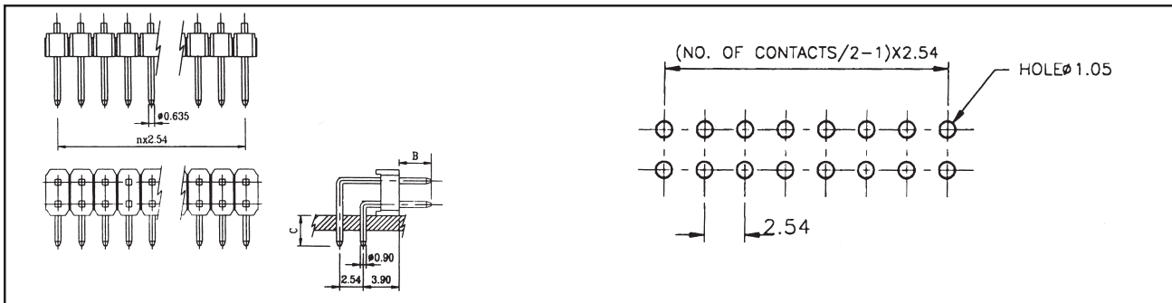
DRAWING - DUAL ROW, RIGHT ANGLE
