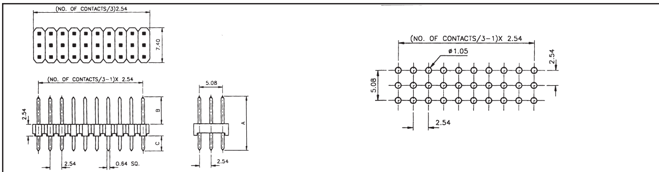
DRAWING - TRIPLE ROW, STRAIGHT
