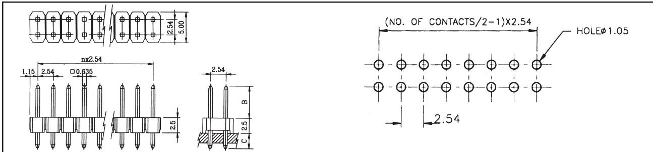
DRAWING - DUAL ROW, STRAIGHT
