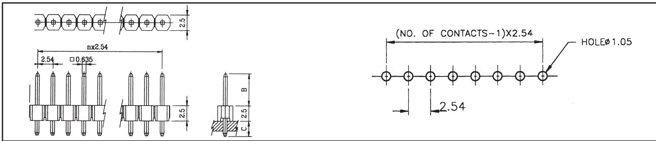
DRAWING - SINGLE ROW, STRAIGHT
