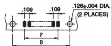
PCB LAYOUT - BOTTOM SIDE
