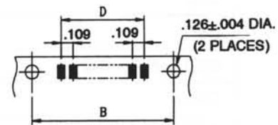
PCB LAYOUT - TOP SIDE
