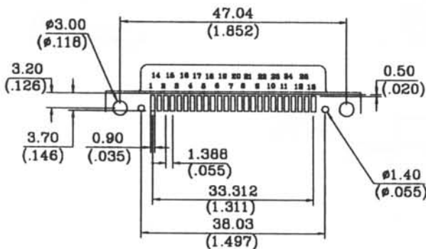
PCB LAYOUT
