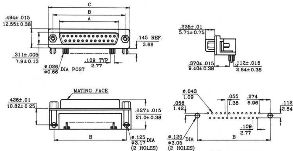
PCB LAYOUT
