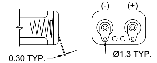
PDSN-10C SOLDER LUGS
