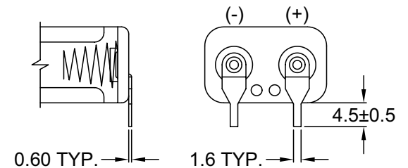
PDSN-10D PCB PINS
