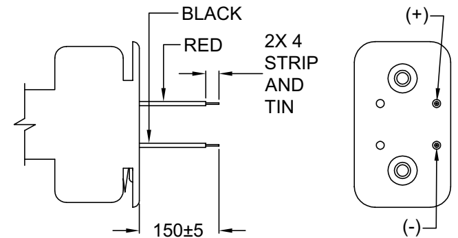
PDSN-20A WIRE LEADS
