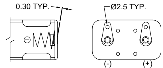
PDSN-20C SOLDER LUGS
