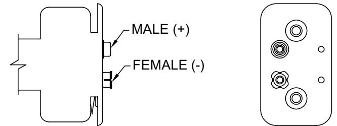
PDSN-20B SNAP TERMINAL
