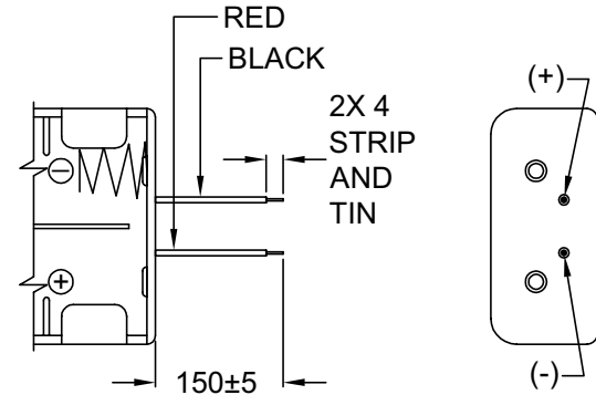
PDSN-28-3A WIRE LEADS
