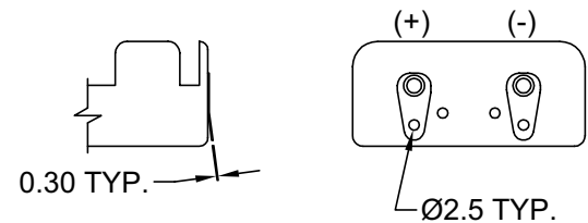
PDSN-28-3C SOLDER LUGS
