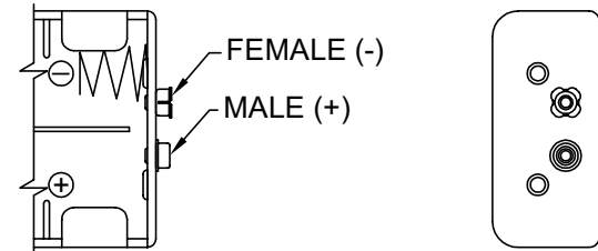
PDSN-28-3B SNAP TERMINAL
