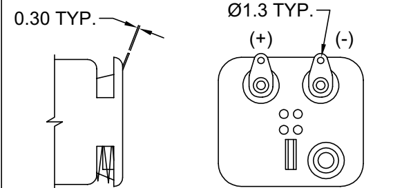
PDSN-38-2C SOLDER LUGS
