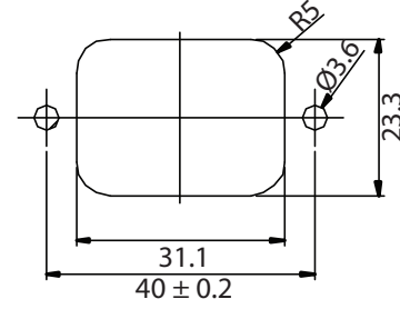
PANEL CUTOUT
